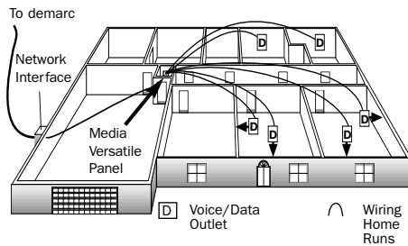
Coax Feed CATV, Satellite or Antenna Media Versatile Panel V Video Outlet Wiring Home Runs
